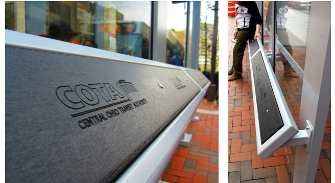
LR-EC-10-HB-C-0 | Column mounted Eclipse leaning rail, powder coated in White Aluminum with Black HDPE slats. All leaning rails with HDPE slats or perforated aluminum are available with routed agency branding as shown here.
